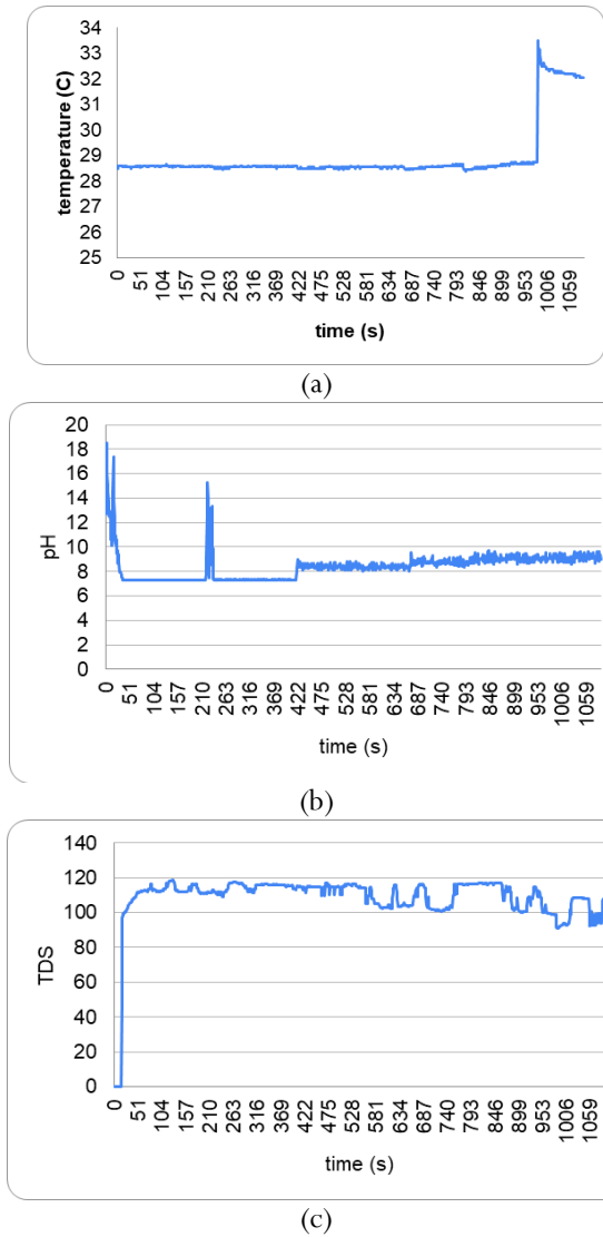
Figure 5. Graph of temperature, pH, and TDS monitoring results over a 1 hour and 17 minutes period (1.059x4s) displayed on Google Sheets.
