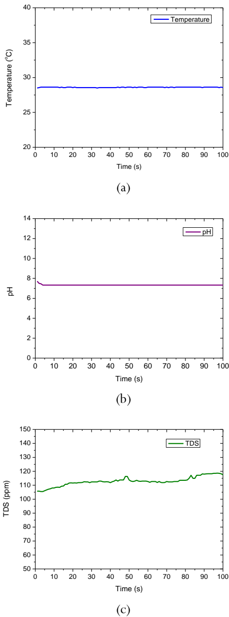
Figure 3. Sensors test results: (a) temperature sensor test, (b) pH sensor test, (c) TDS sensor test.
