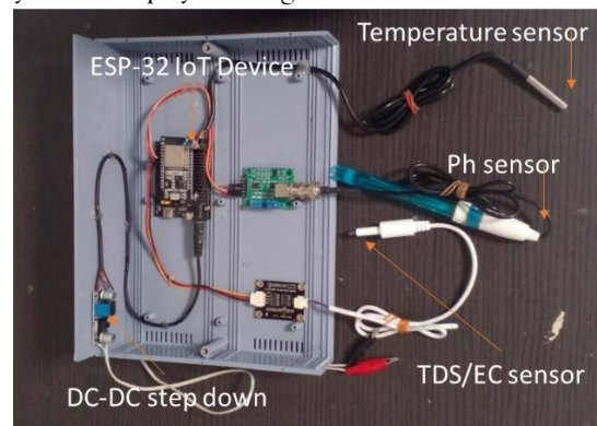
Figure 2. The hardware of IoT-based water quality measurement
